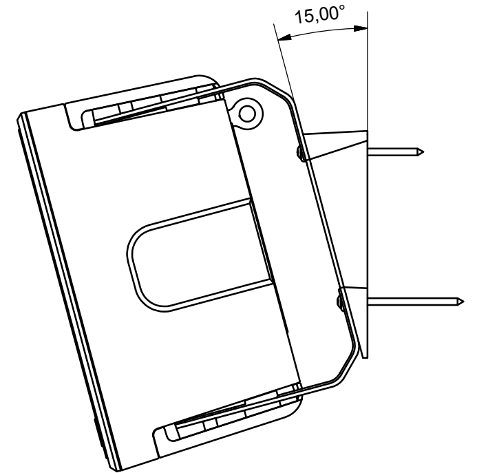
WITH OPTIONAL ANGLE BLOCK
